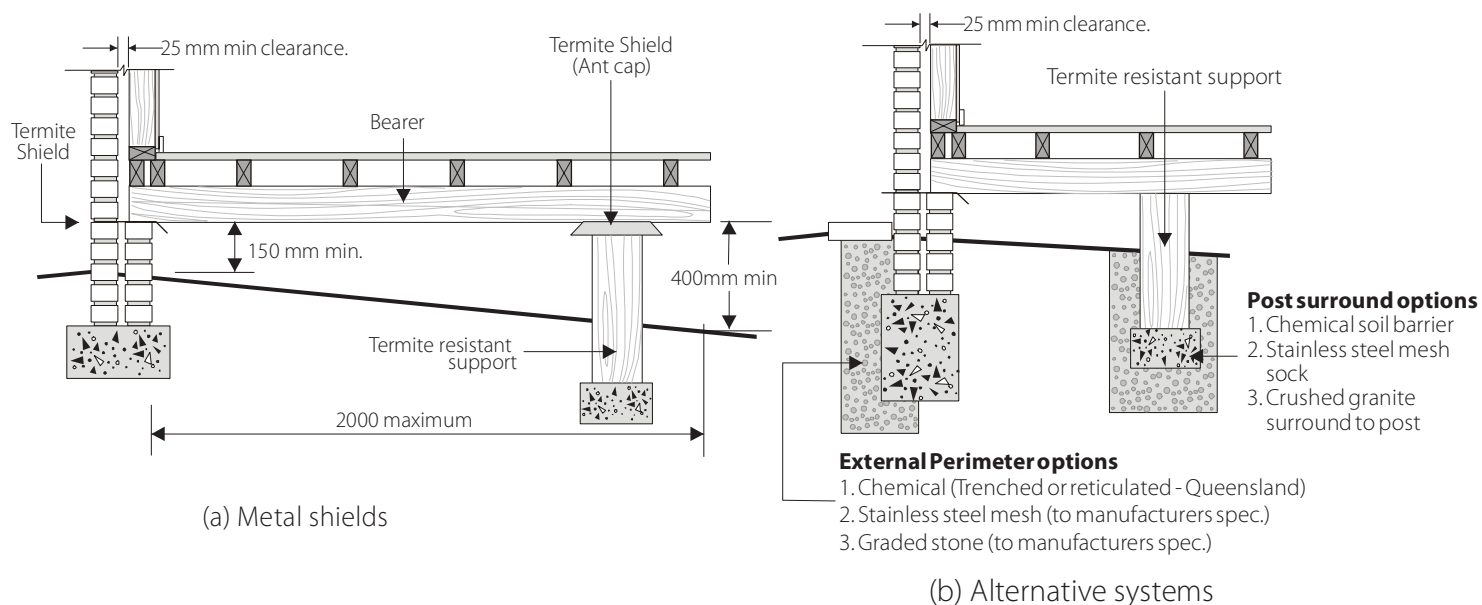
FIGURE 3 TERMITE MANAGEMENT SYSTEMS FOR SUSPENDED TIMBER FLOORS
