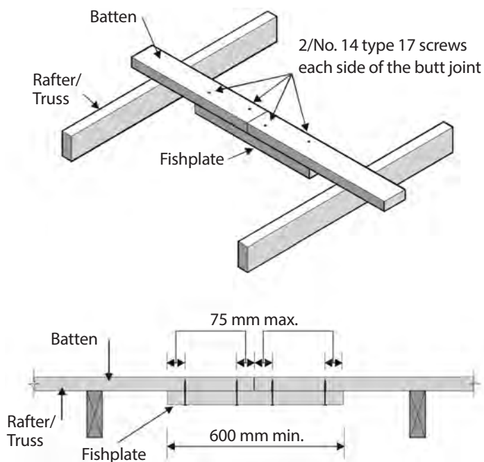
Figure 2 – Joining battens between supports
