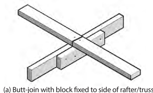
Figure 1 – Joining battens at supports
