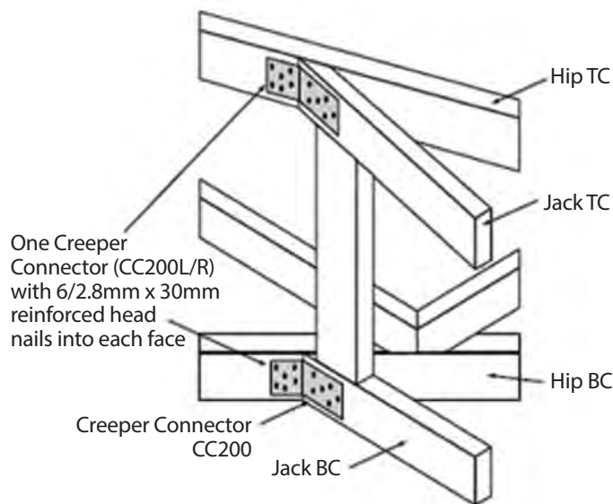
Figure 3 – Typical jack to hip truss connection as specified in AS 4440 for N4, C2 and C3 Wind Classifications
