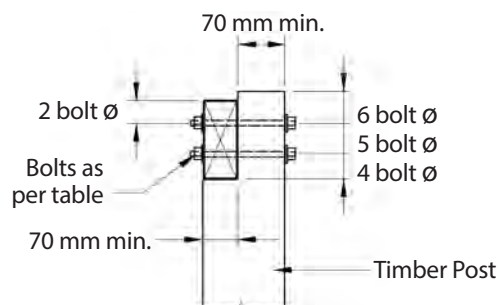
Figure 4 – Example 1 - 1684 typical beam to post detail
