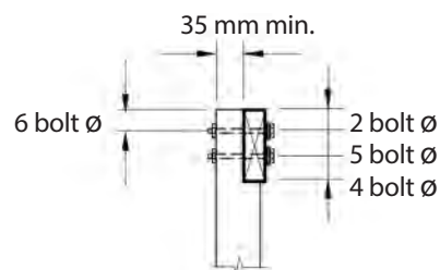
Figure 5 - Example 2 - 1684 typical beam to post detail
