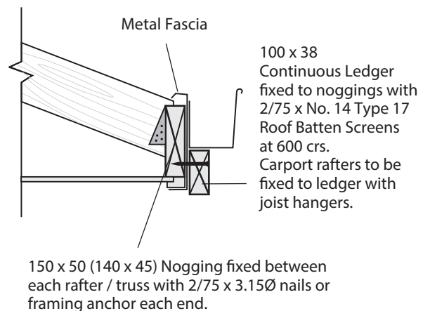
Figure 6 – Strengthening metal fascias to attach pergola rafters
