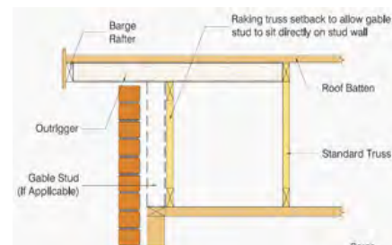
OUTRIGGERS
