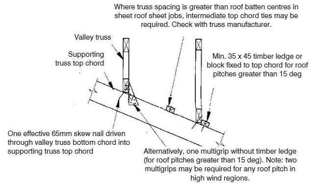
FIXING DETAILS FOR VALLEY TRUSSES
