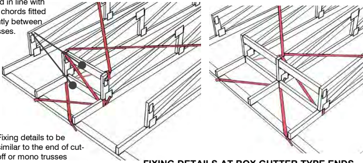
FIXING DETAILS AT BOX GUTTER TYPE ENDS
