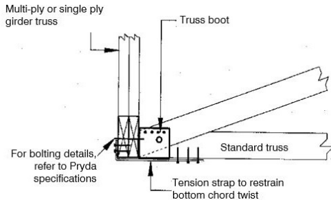
STANDARD TRUSS BOOT AND ANTI-TWIST BAR
