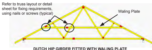
DUTCH HIP GIRDER FITTED WITH WALING PLATE
