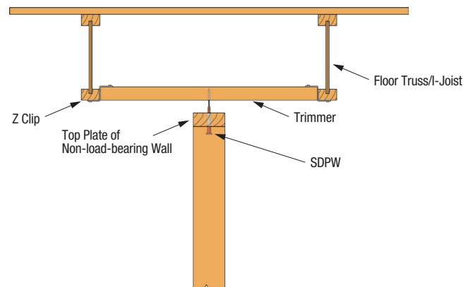
SDPW Wall Plate to Floor Truss/I-Joist Installation
