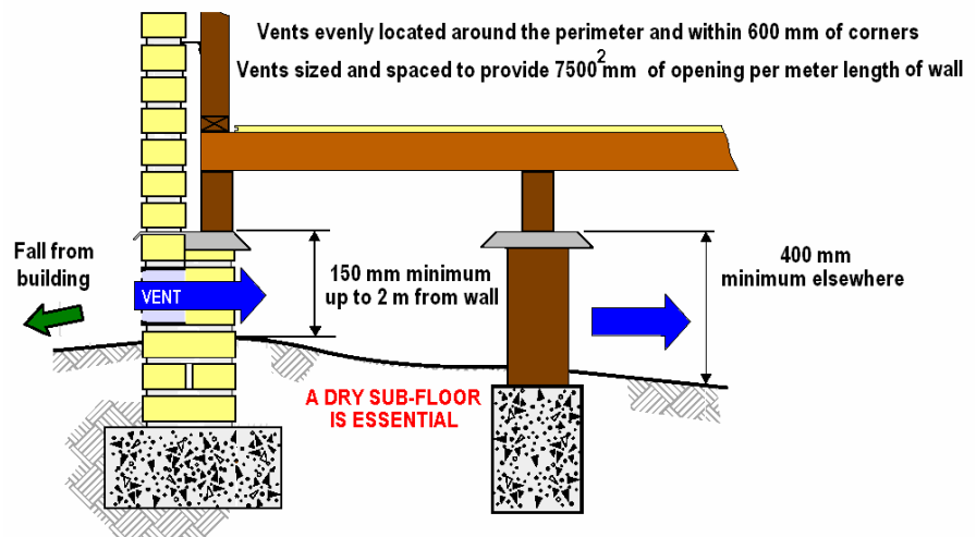
Figure 3a – Sub-floor Ventilation
