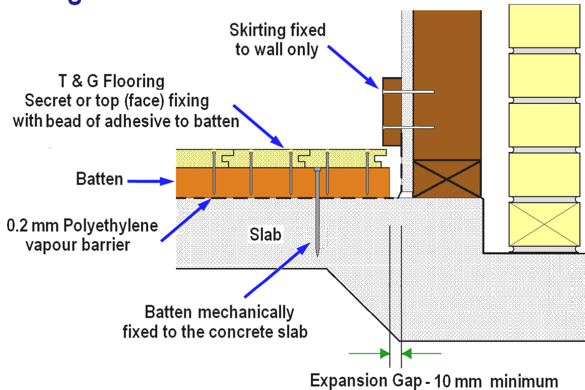
Figure 3i - Details of fixing in battens
