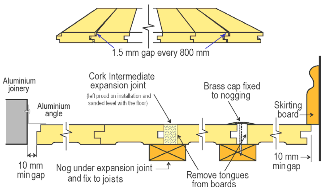
Figure 3c – Expansion Gap details
