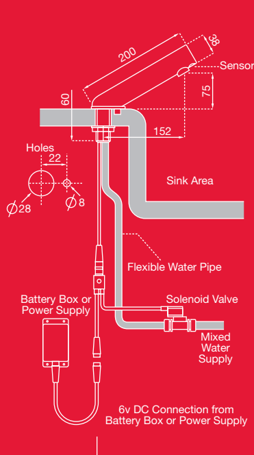
Deck Mounted Diagonal. Models 42208 and 42211. Brushed stainless steel.
