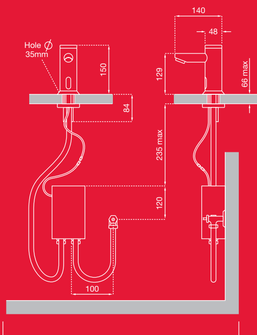
Deck Mounted Vertical. Models 42220 and 42221. Polished Chrome Brass.
