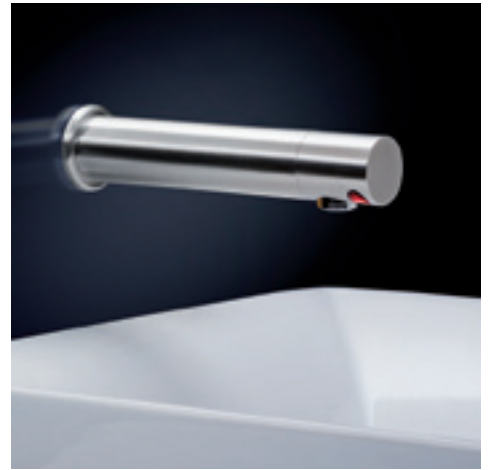
Wall Mounted Short. Models 42223 and 42222. Brushed stainless steel.
